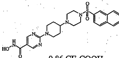
.086 CF 3 COOH compound 4
